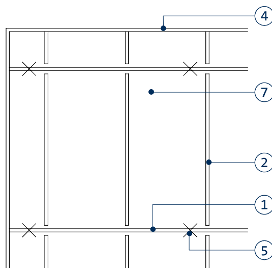
Layout 2 - module standard 600 x 1200 mm
