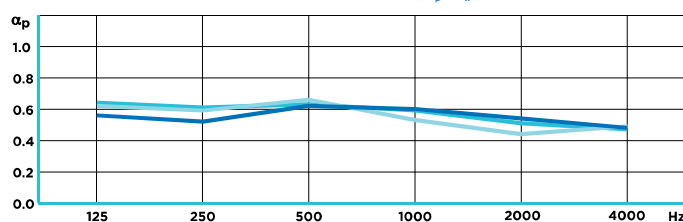
ABSORBTIA ACUSTICA ( \alpha_p | \alpha_w )
