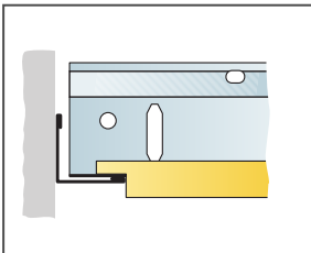
Tegular rebate with angle trim.
