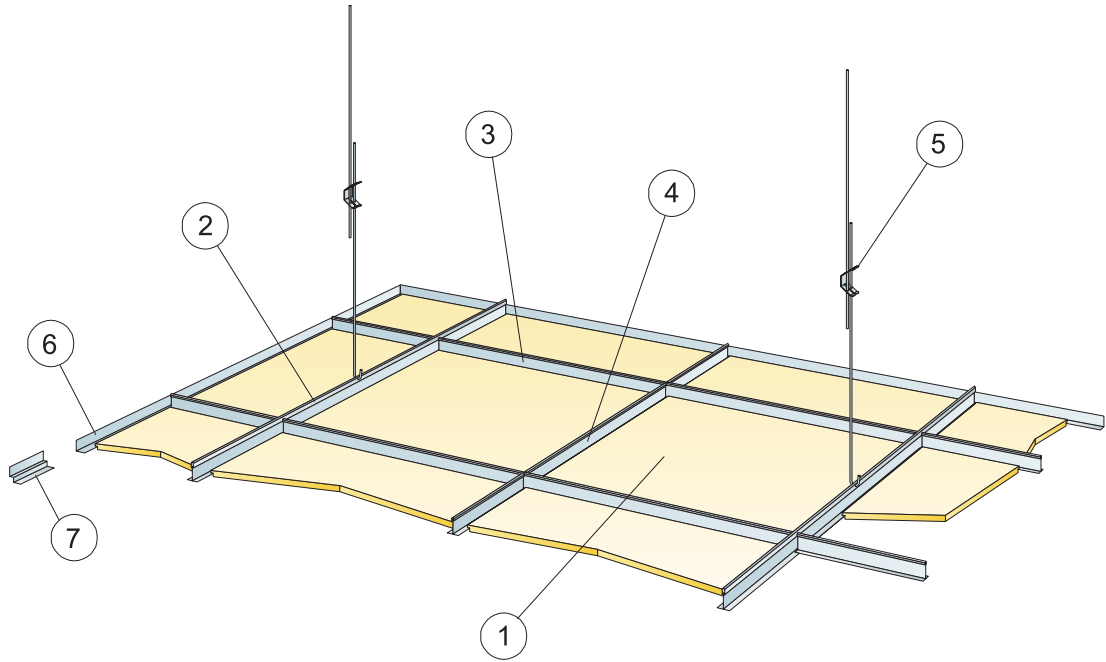
Installation diagram (M140) for Ecophon Opta E
